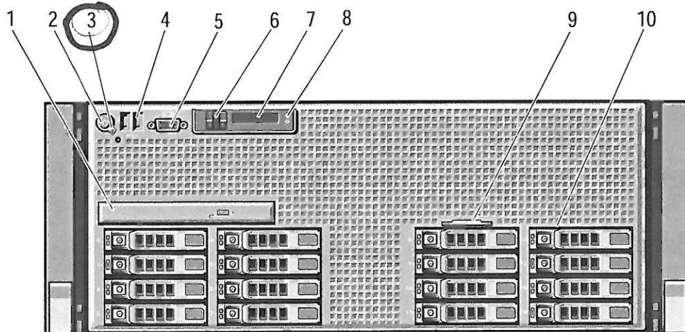
Front-Panel Features and Indicators
